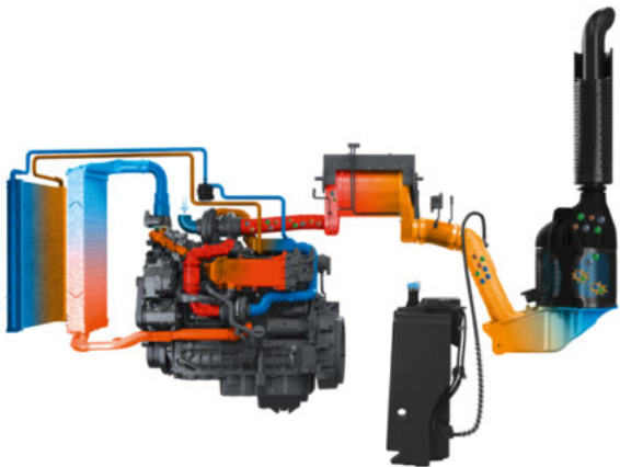
The high-grade solution for extremely low operating costs: the combination of external exhaust gas recirculation (AGRex), passive diesel particulate filter (CSF) and SCR technology.
